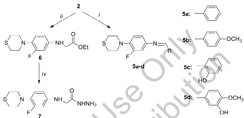
Scheme 2. Reaction and conditions for the synthesis of compounds 5-7. i : benzaldehyde (for 5a), 4-methoxybenzaldehyde (for 5b), 2-hydroxybenzaldehyde (for c), 3-hydroxy-4-methoxybenzaldehyde (for 5d) in absolute EtOH, reflux, 20-22 h (Method 1) or 5 min., 150 W (Method 2); ii : \text{BrCH}_2\text{CO}_2\text{Et} in THF, TEA, rt., 18 h (Method 1) or \text{BrCH}_2\text{CO}_2\text{Et} , TEA, 5 min., 100 W (Method 2); iv : \text{H}_2\text{NNH}_2 \cdot \text{H}_2\text{O} in EtOH, reflux, 18 h (Method 1) or \text{H}_2\text{NNH}_2 \cdot \text{H}_2\text{O} , 10 min., 150 W (Method 2).
