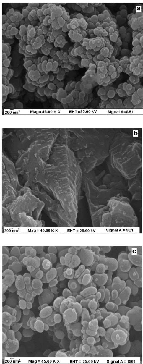
FIG. 8 SEM images of a \text{PVF}^+\text{ClO}_4^- , b PANI and c \text{PVF}^+\text{ClO}_4^- -PANI composite coatings
