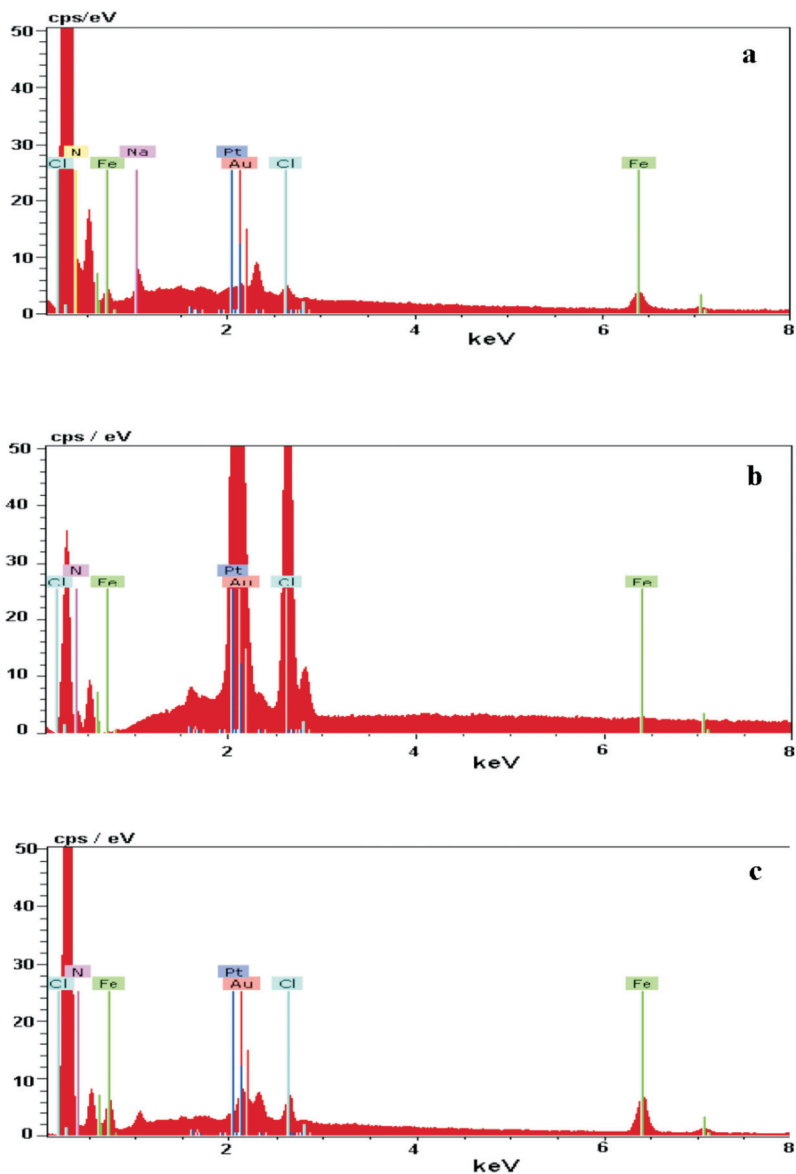
FIG. 9 EDS spectra of a) PVF + ClO 4 - , b) PANI and c) PANI-PVF + ClO 4 - composite coatings
