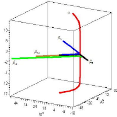
Figure 2. Smarandache curves of a spacelike curve with timelike binormal
