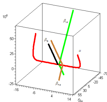
Figure 5. Smarandache curves of a null curve.
