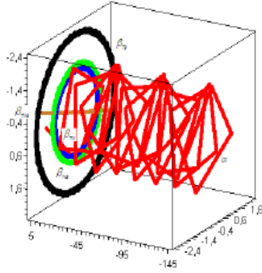
Figure 1. Smarandache curves of a timelike curve
