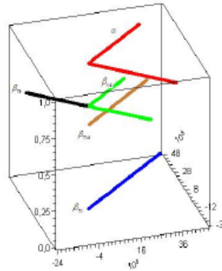
Figure 4. Smarandache curves of a planar spacelike curve with timelike principal normal
