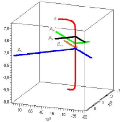
Figure 3. Smarandache curves of a nonplanar spacelike curve with timelike principal normal
