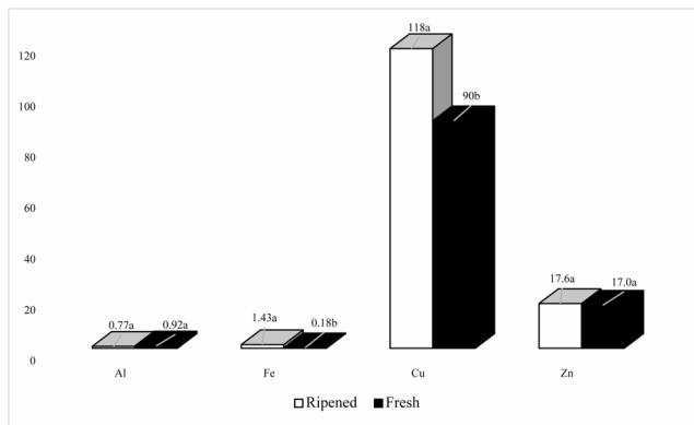
Fig. 1 Statistical comparison of PTM levels (median) in cheeses classified by ripening stage. Al, Fe, and Zn: mg/kg wet weight; Cu: µg/kg wet weight
