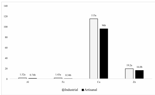
Fig. 3 Statistical comparison of PTM levels (median) in cheeses classified by production type. Al, Fe, and Zn: mg/kg wet weight; Cu: µg/kg wet weight
