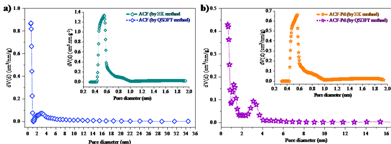
Fig. 3 The pore size distribution of ACF and ACF-Pd
