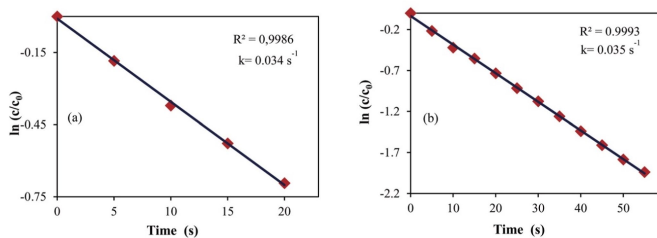
Fig. 13 Plots of \ln(c/c_0) versus reaction time for catalytic reductions of (a) MO and (b) RhB dyes in the presence of AC-Pd
