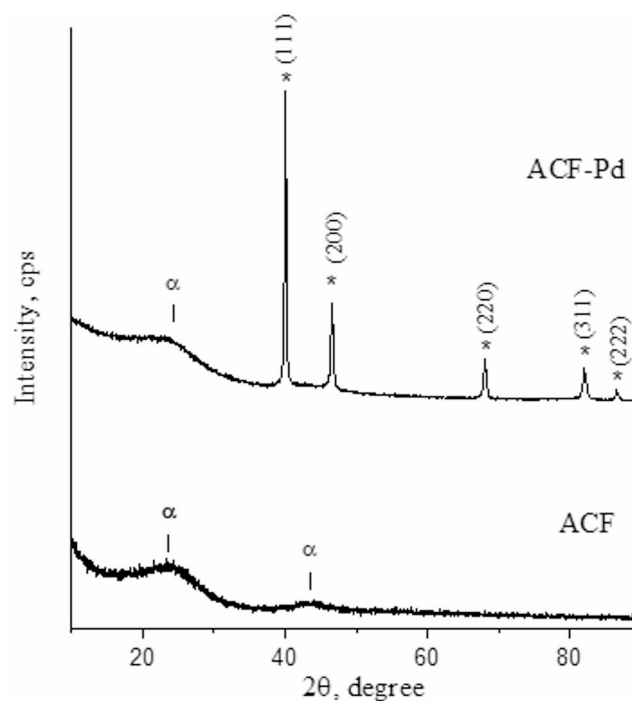
Fig. 6 XRD pattern of ACF-Pd (*: Pd(0), \alpha : carbon)
