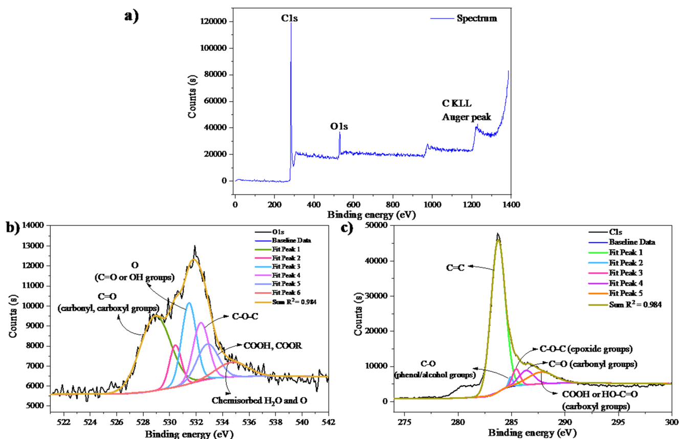
Fig. 5 Deconvolution of ACF; (a) general spectrum (b) C1s spectra, (c) O1s spectra
