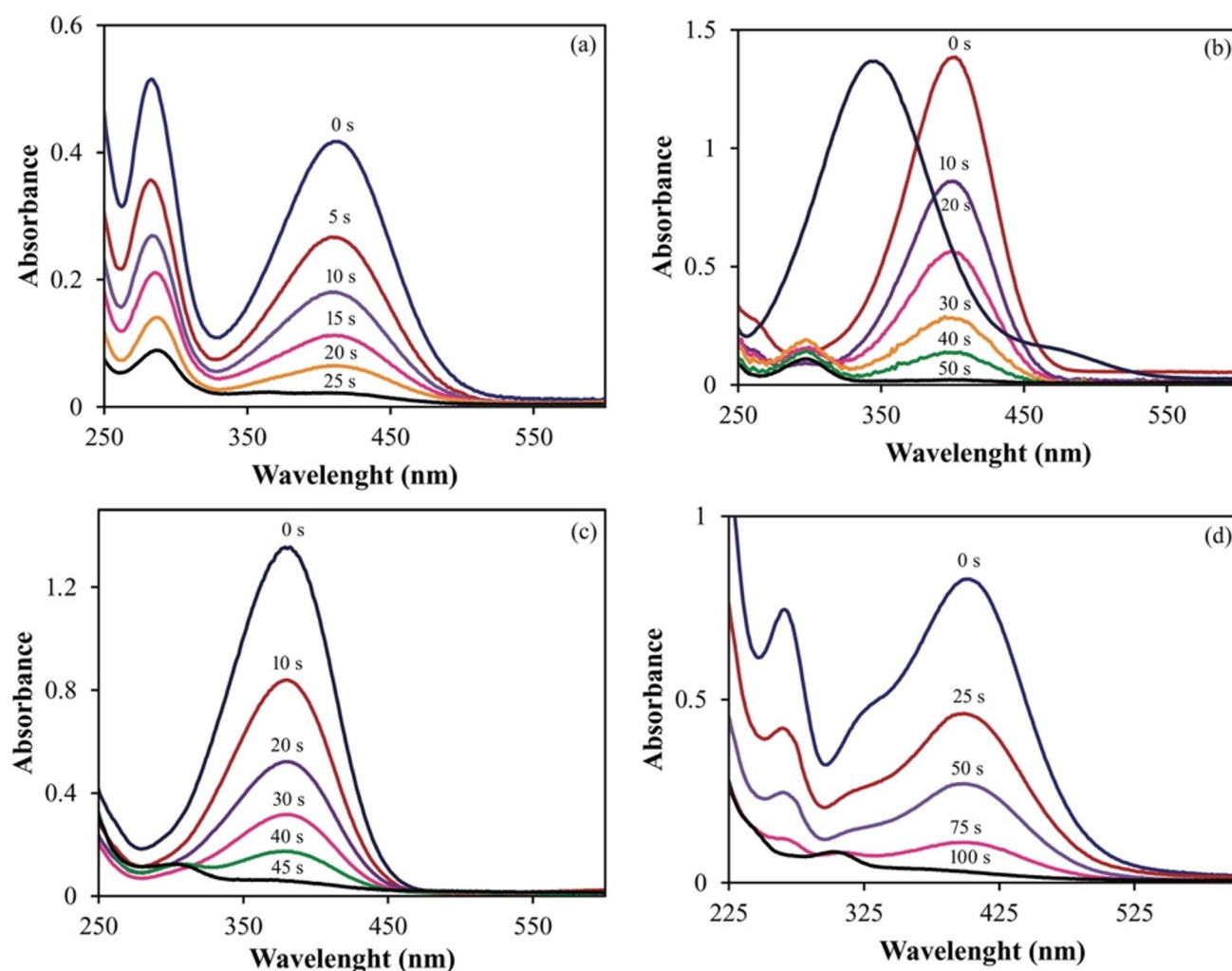
Fig. 9 UV-Vis spectra of the catalytic reductions of (a) 2-NA, (b) 4-NP, (c) 4-NA and (d) 4-NPD in the presence of AC-Pd
