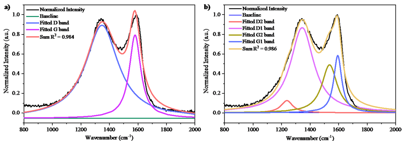
Fig. 4 Deconvolution of Raman spectra into (a) 2 peaks, (b) 4 four peaks of ACF
