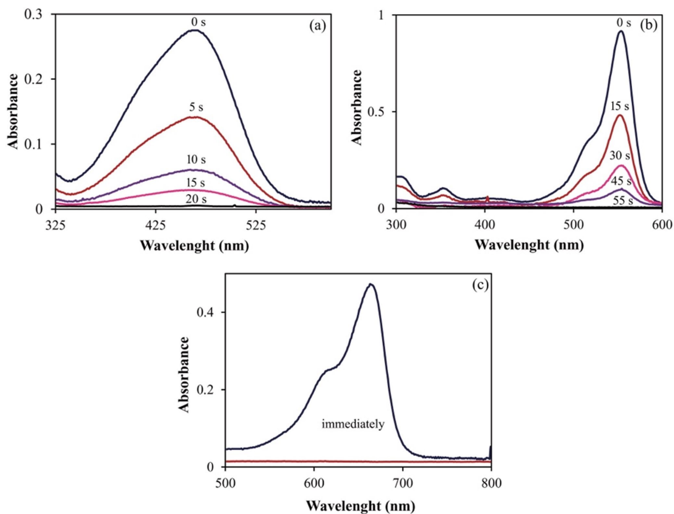
Fig. 12 UV-Vis spectra of the catalytic reductions of organic dyes (a) MO (b) RhB and (c) MB in the presence of AC-Pd
