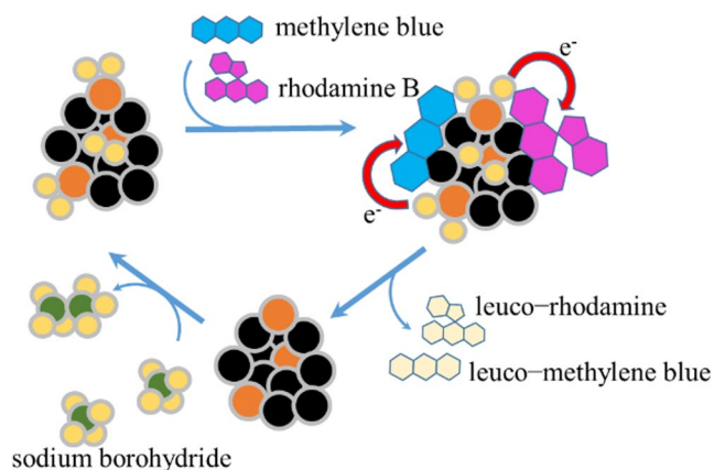
Fig. 11 Proposed reaction mechanism for catalytic conversion of methylene blue and rhodamine B to leuco-derivatives
