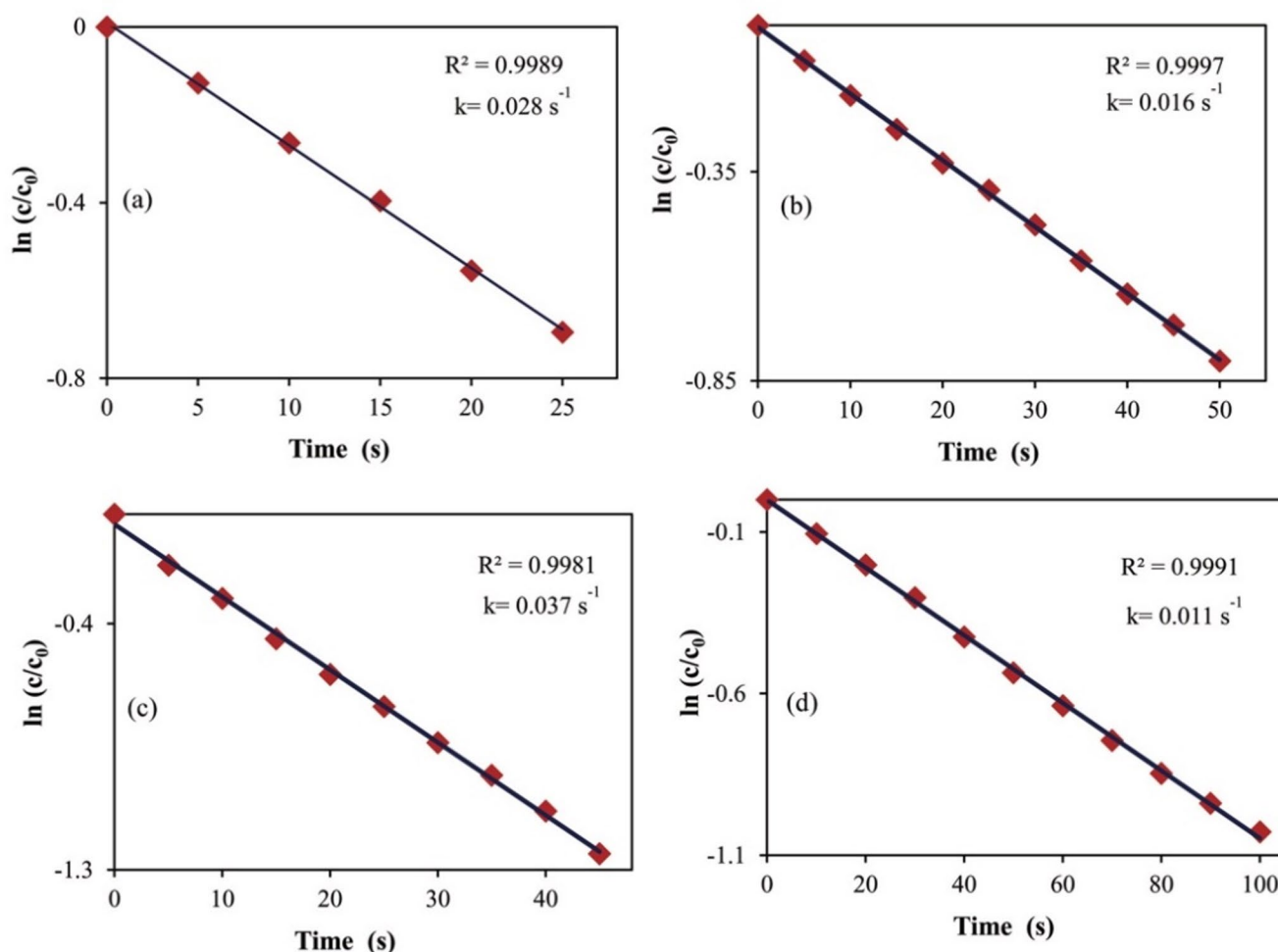
Fig. 10 Rate constants for the catalytic reductions of 2-NA (a), 4-NP (b), 4-NA (c), and 4-NPD (d) using ACF-Pd catalyst
