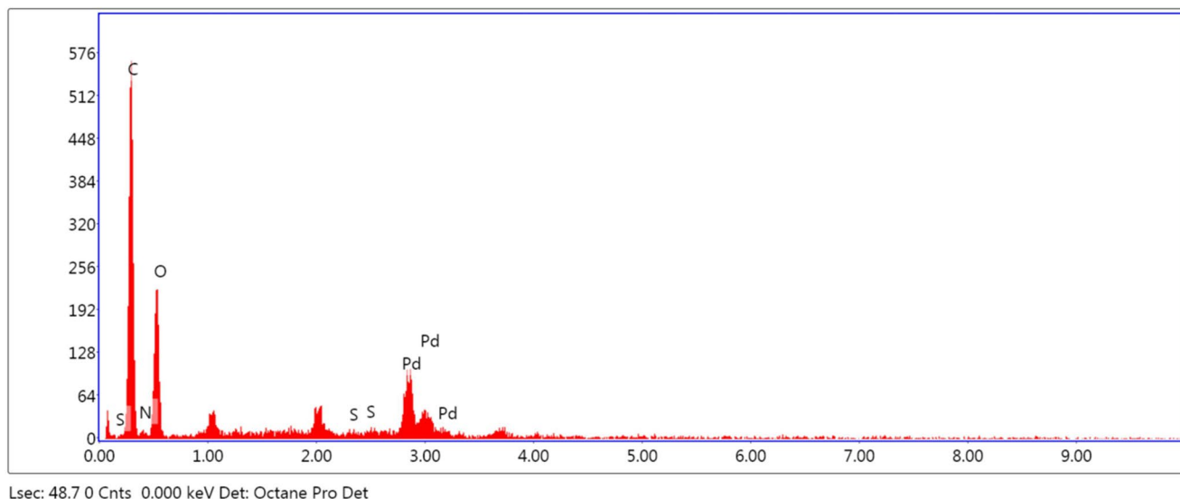
Fig. 15 EDS spectrum of used ACF–Pd catalyst
