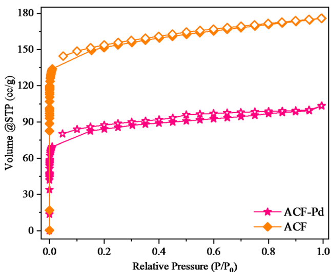
Fig. 2 \text{N}_2 adsorption/desorption isotherms of ACF
