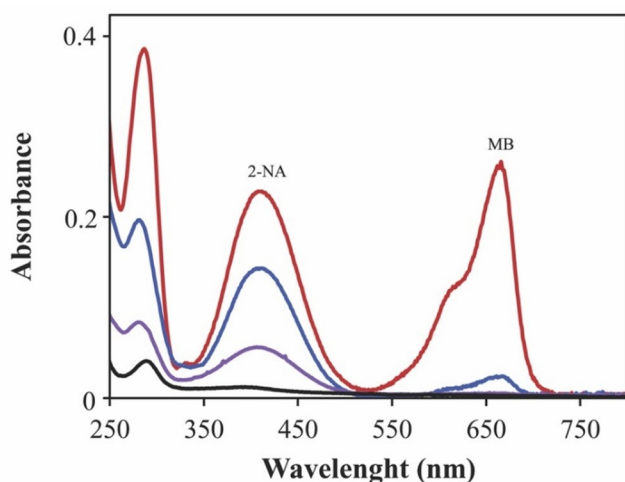
Fig. 14 UV-Vis spectrum of catalytic reduction of [2-NA+MB] mixture using ACF-Pd catalyst
